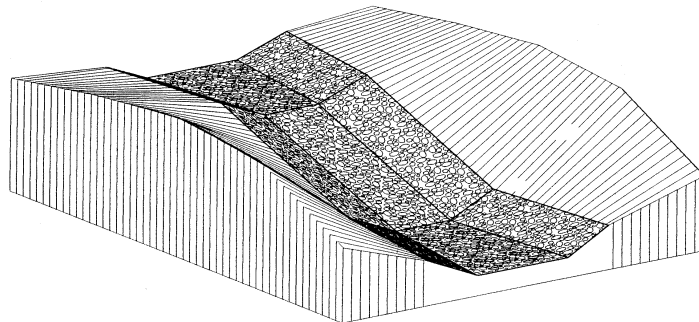
ROCK CHUTE - ISOMETRIC VIEW
