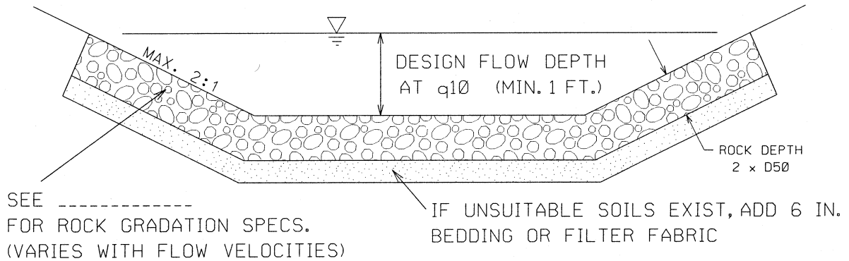
CROSS SECTION OF ROCK LINED CHANNEL / CHUTE
