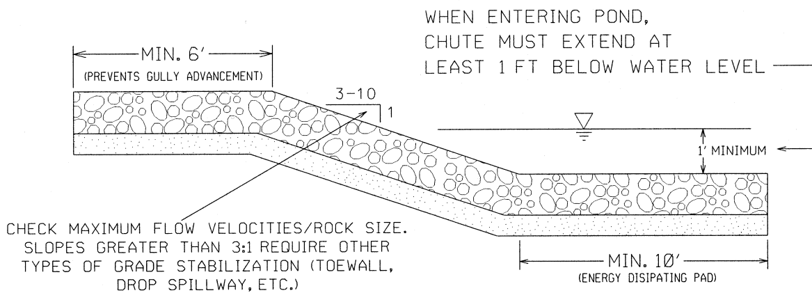
PROFILE FOR ROCK CHUTE
